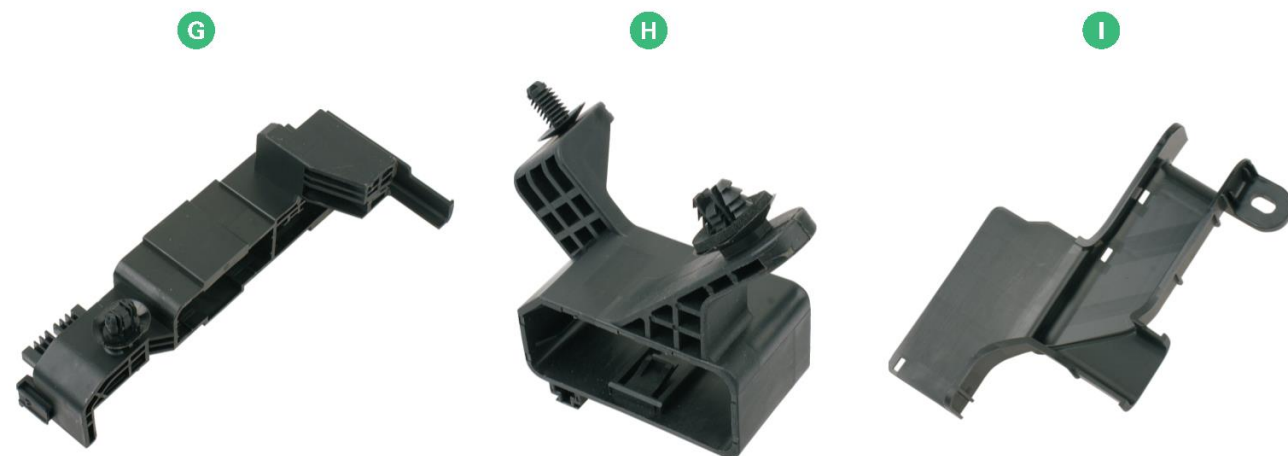
HD-K-P02R-1: 170.6 × 76.1 × 84.5 HD-G-P03B: 101.3 × 98.7 × 35.9 HDFA-G-P01: 169.3 × 116.3 × 76.3
